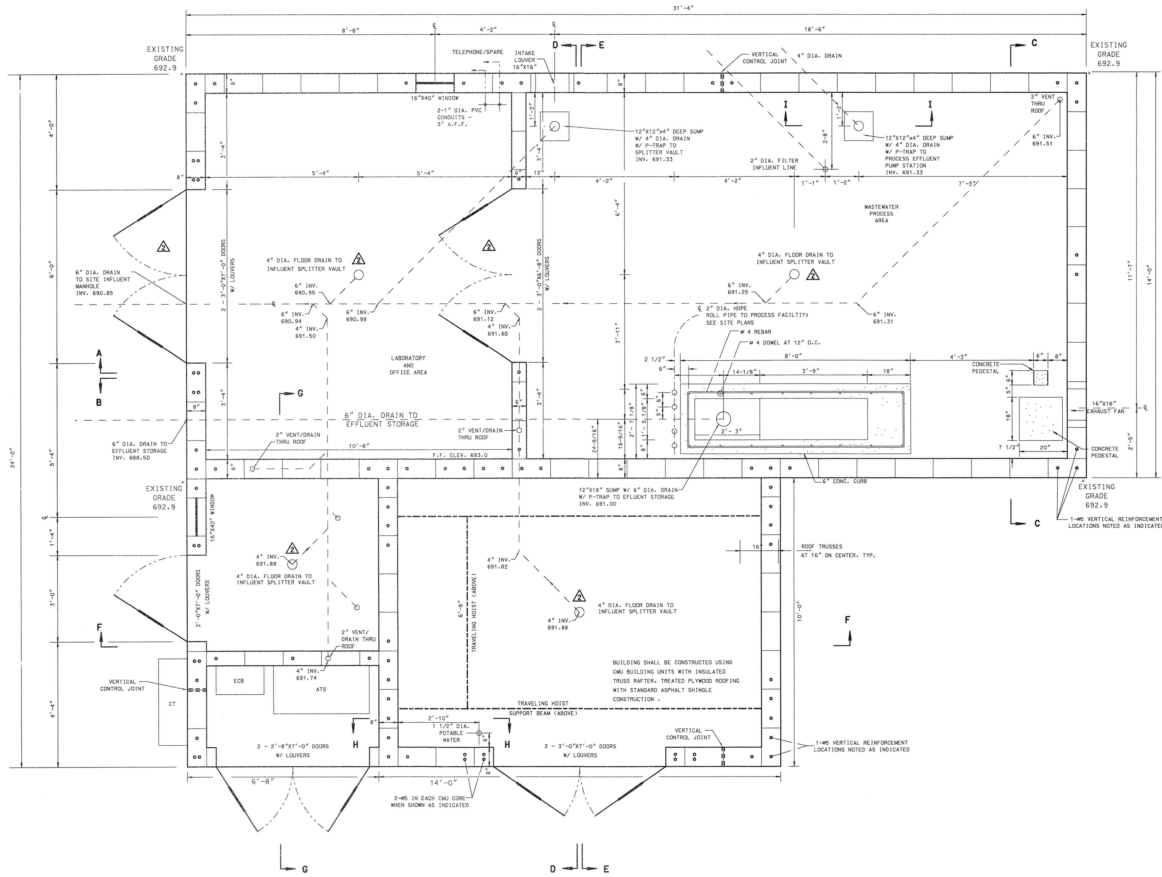
WASTEWATER FACILITIES BUILDING SCALE: 1/2" = 1'-0"
