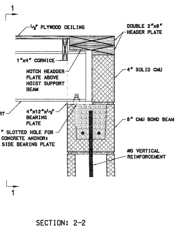
SECTION: 2-2
